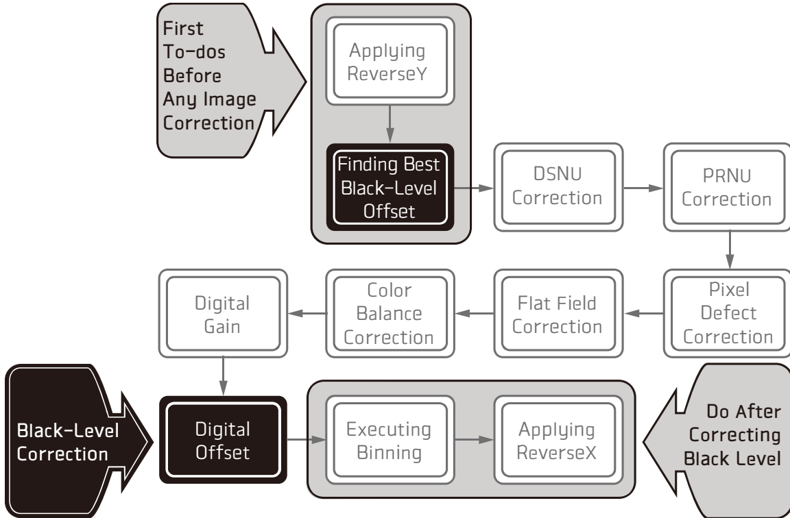
Figure 9-8 Sequence of signal processing and Black Level
