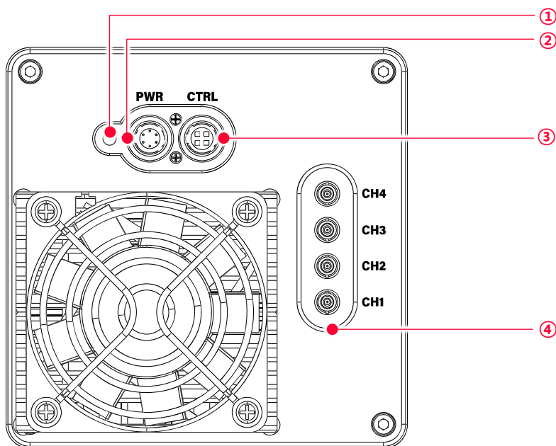
Figure 7-1 VP-103MX2-M/C24I Back Panel
