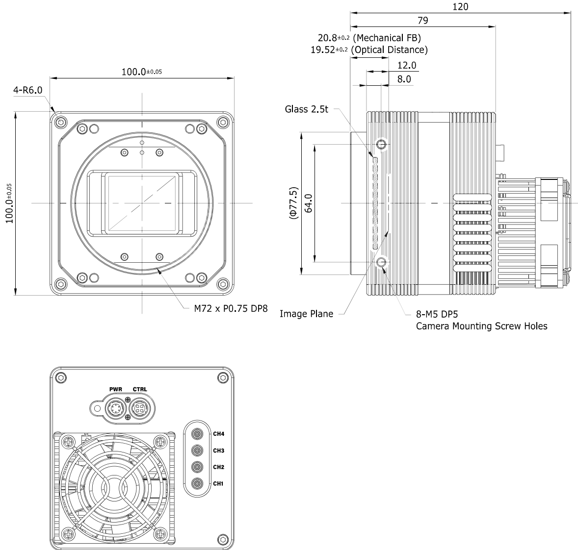
Figure 5-3 VP-103MX2-M/C24I Mechanical Dimension
