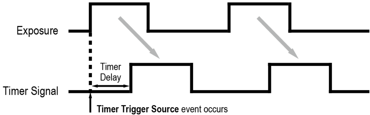
Figure 9-16 Timer Signal
