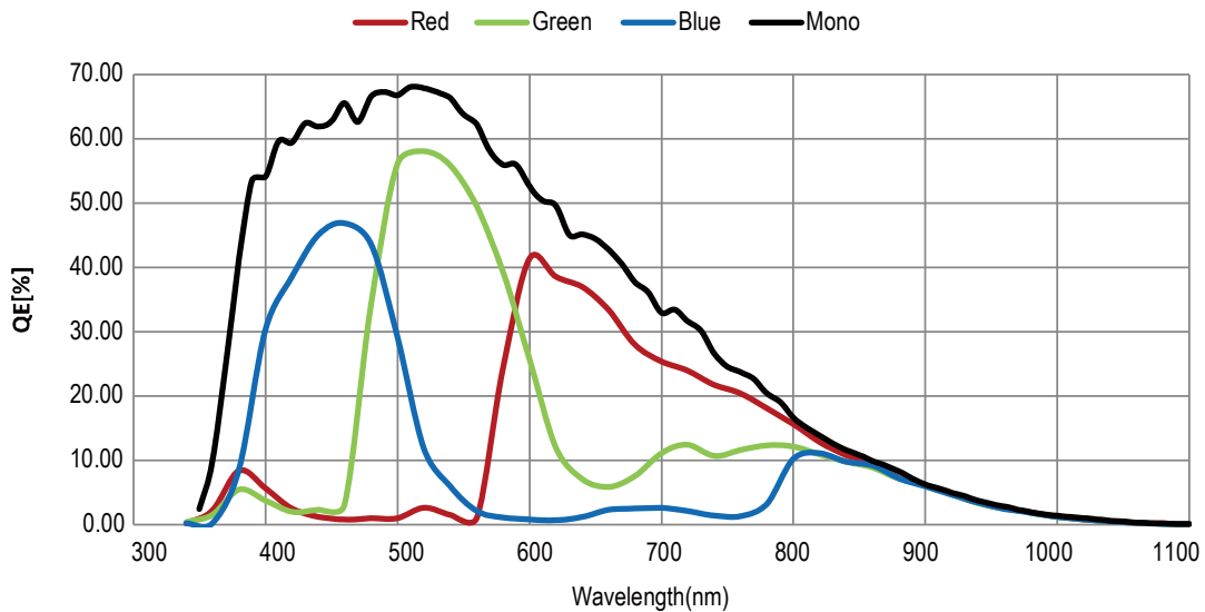
Figure 5-2 Spectral Response
