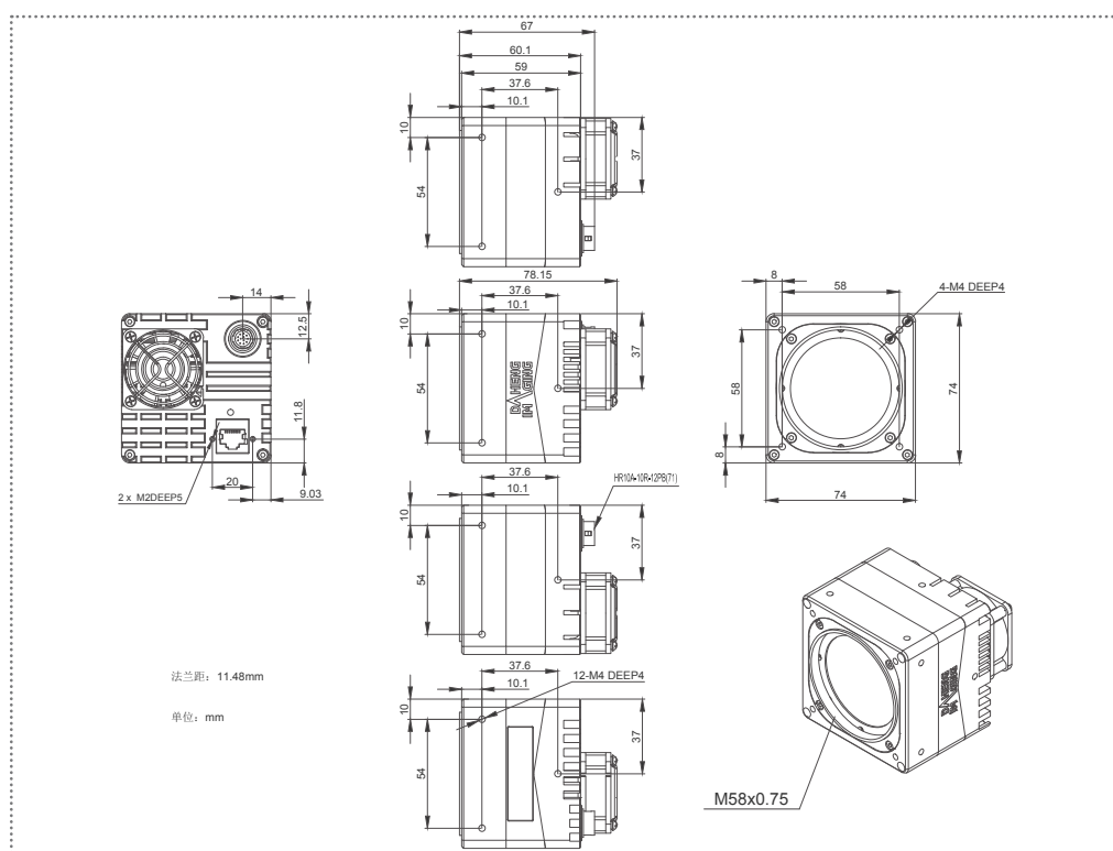
MARS-5000-24GTM/C-NF M58-D1, M58 □ (法兰距 11.48mm)
