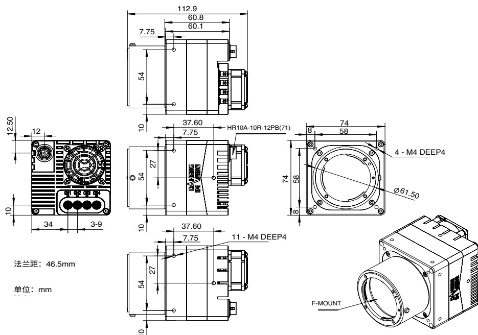
MARS-513-940X2M/C-NF (F □)
