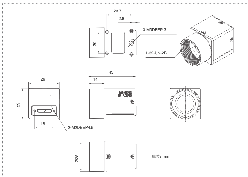
MER2-041-608U3M/C-L-HS-6P
