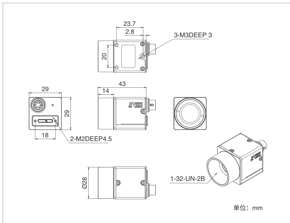
MER2-041-608U3M/C-HS-6P
