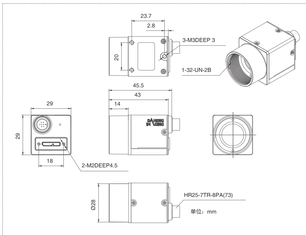
MER2-502-79U3M/C-HS
