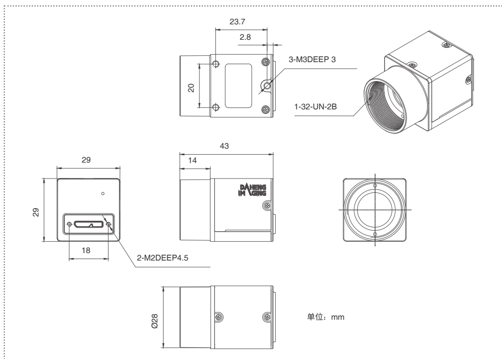
MER2-502-79U3M/C-L-HS
