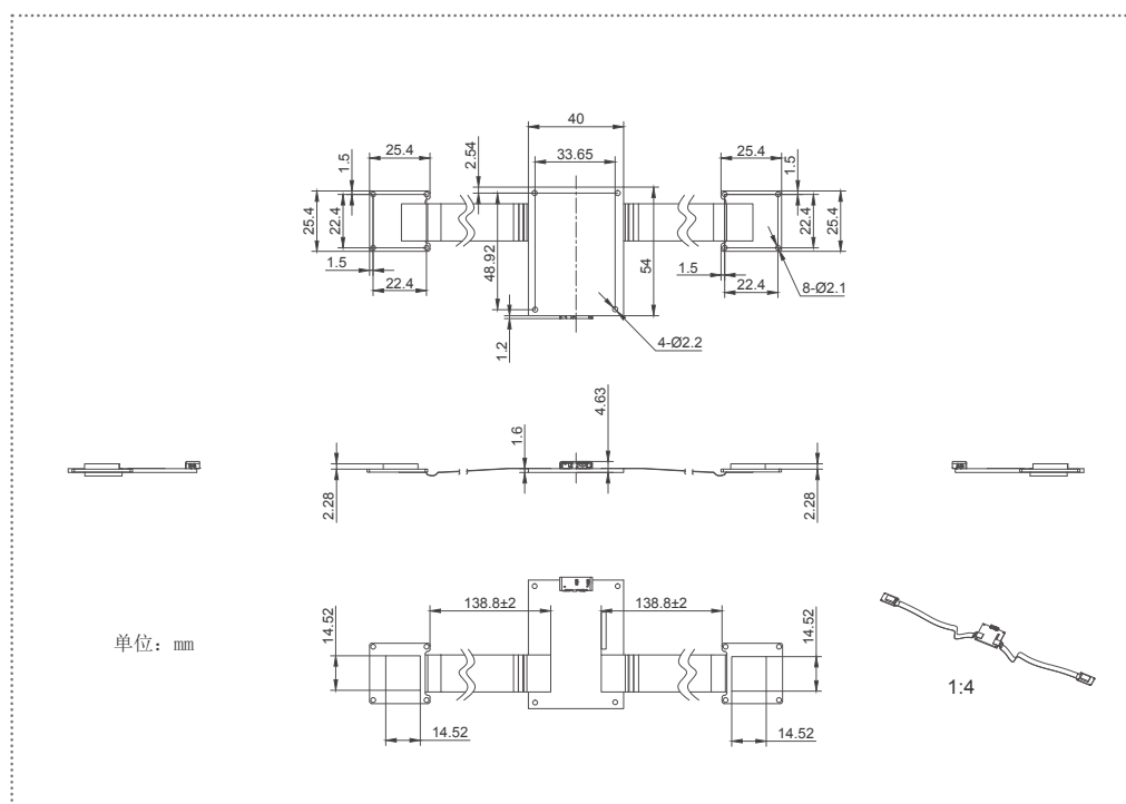
VEN-134-90U3M/C-D, No-mount
