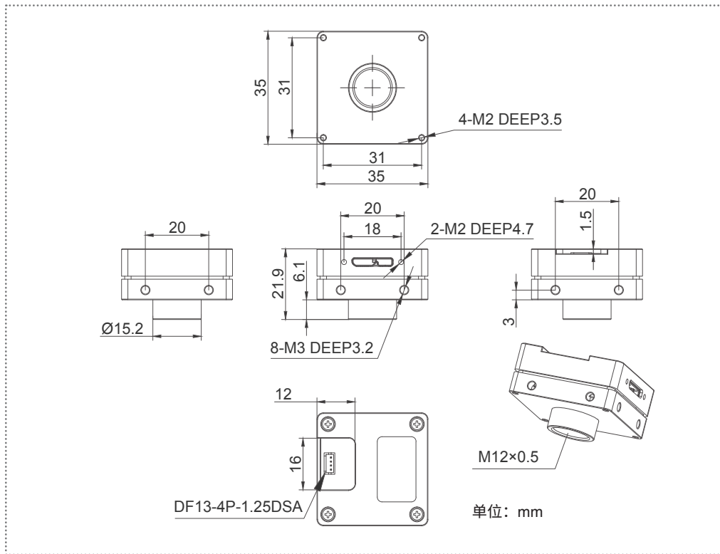
VEN-161-61U3M/C, S 口
