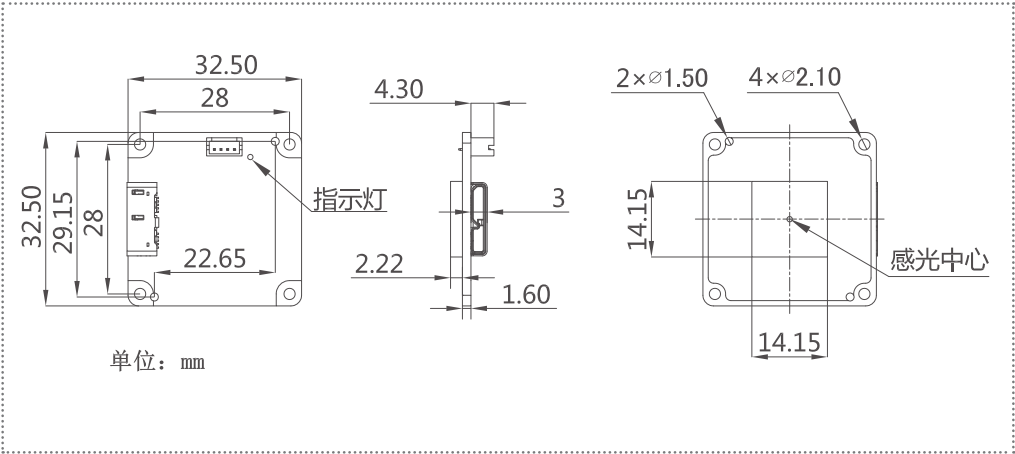
VEN-161-61U3M/C, No-mount
