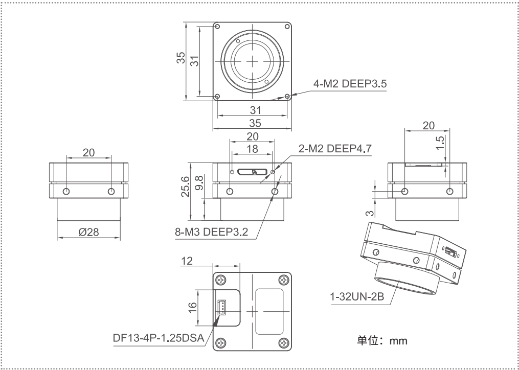
VEN-161-61U3M/C, C 口
