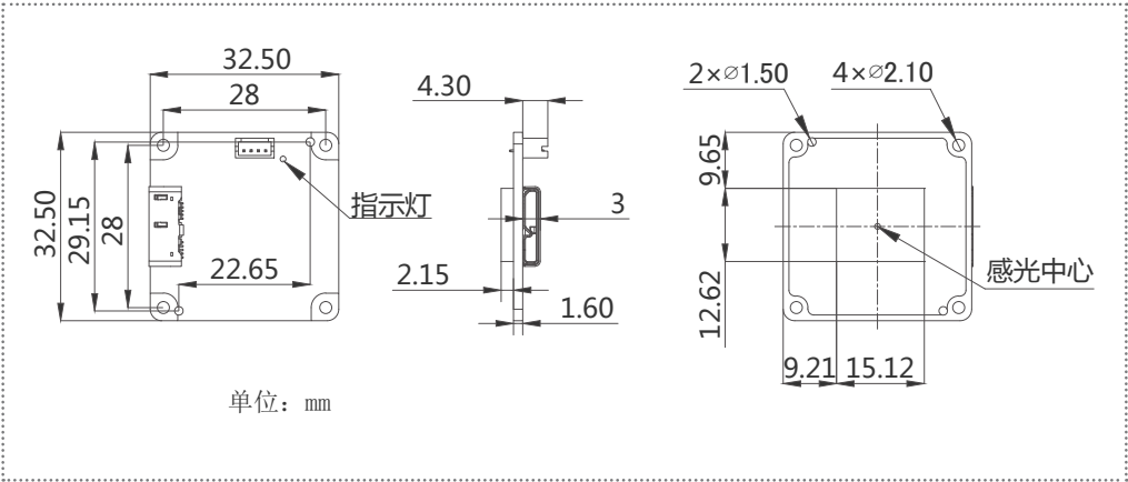
VEN-830-22U3M/C, No-mount
