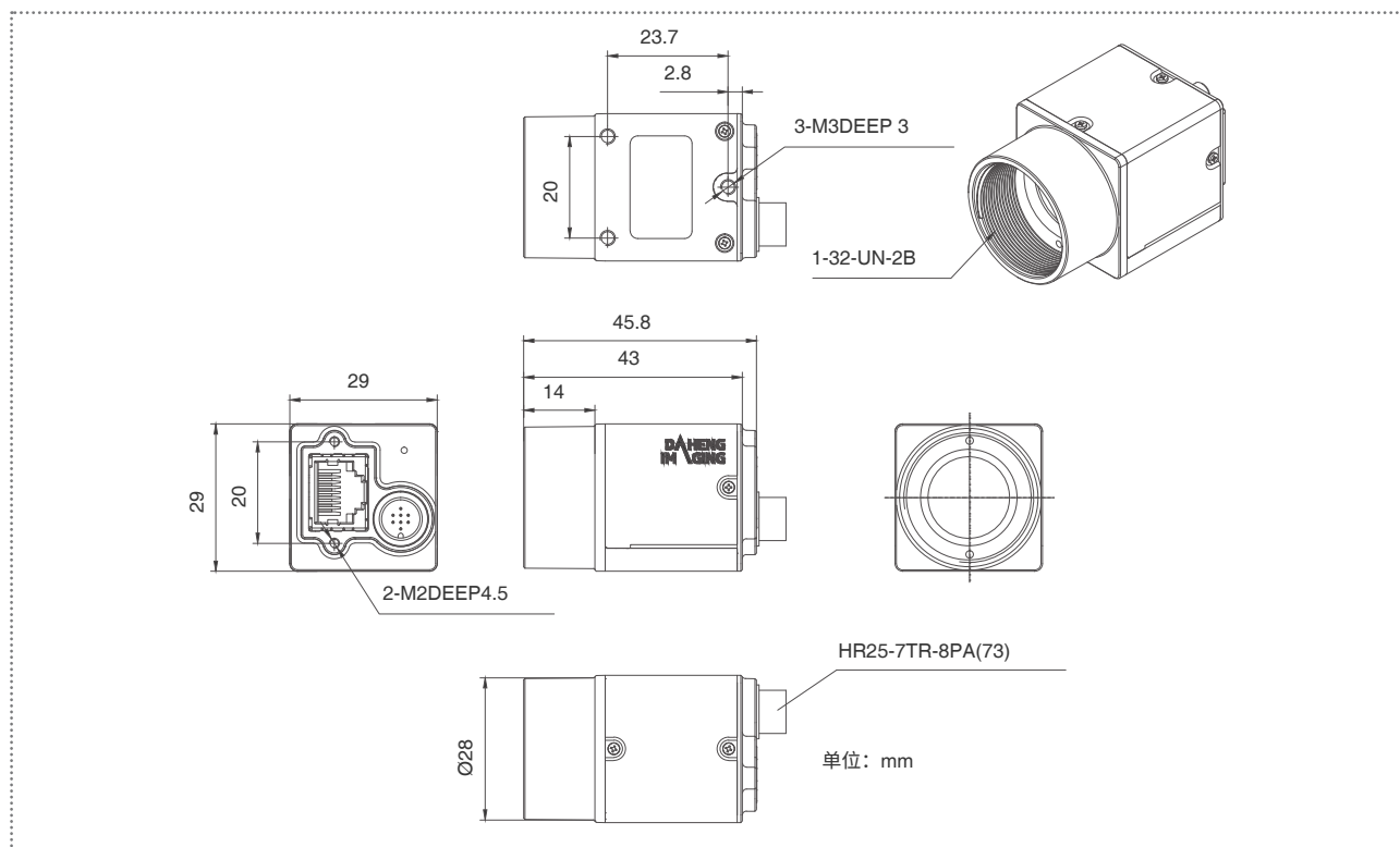
MER2-501-23GM/C
