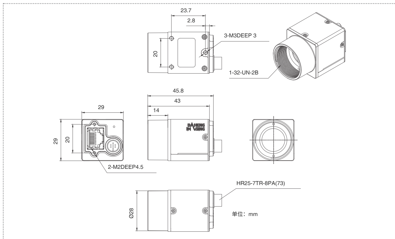
MER2-160-75GM/C
