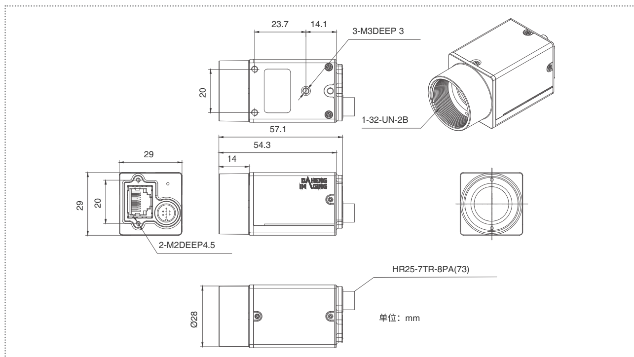
MER2-160-75GM/C-P
