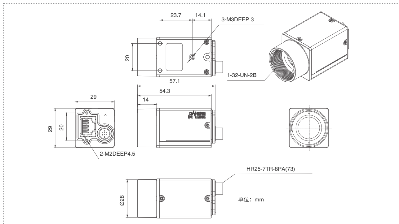
MER2-302-37GM/C-P
