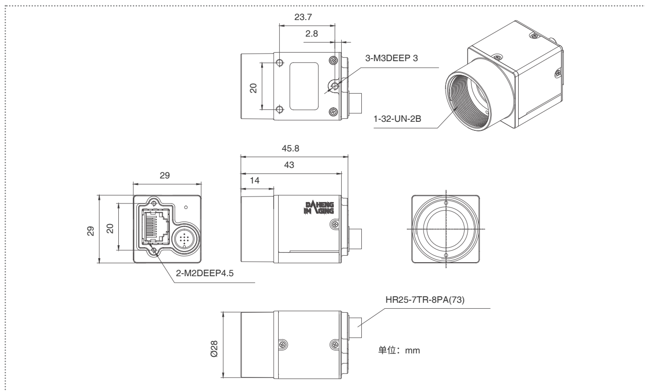
MER2-302-37GM/C
