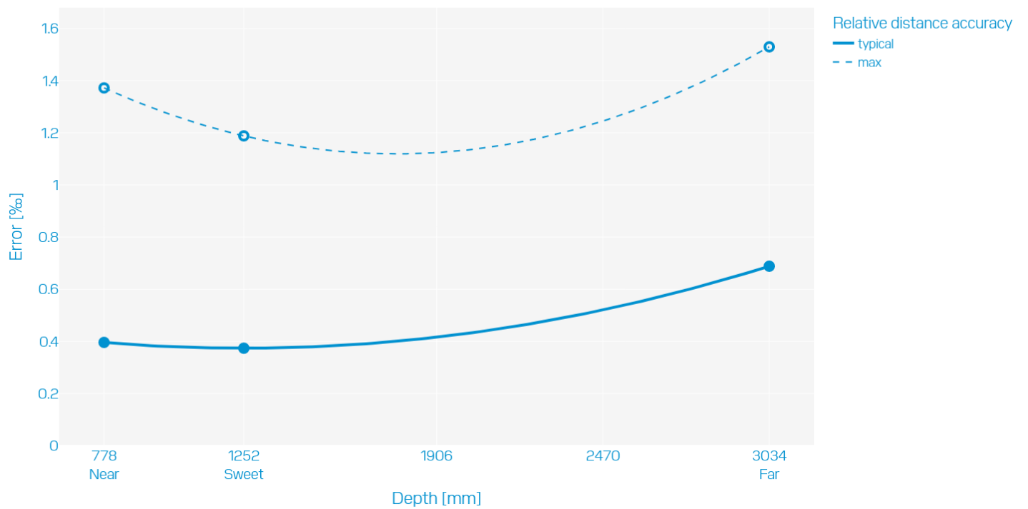
Relative distance accuracy - Camera mode MotionCam-3D L
