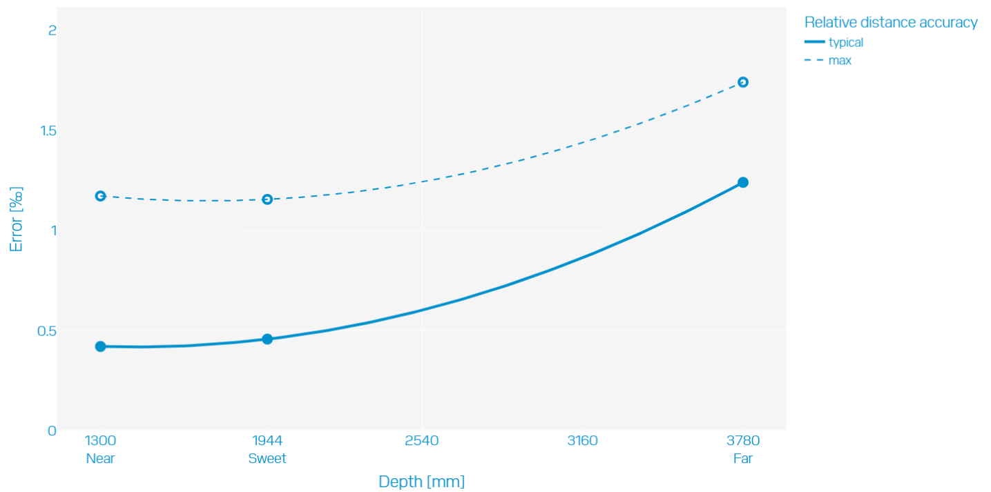
Relative distance accuracy - Scanner mode MotionCam-3D L+
