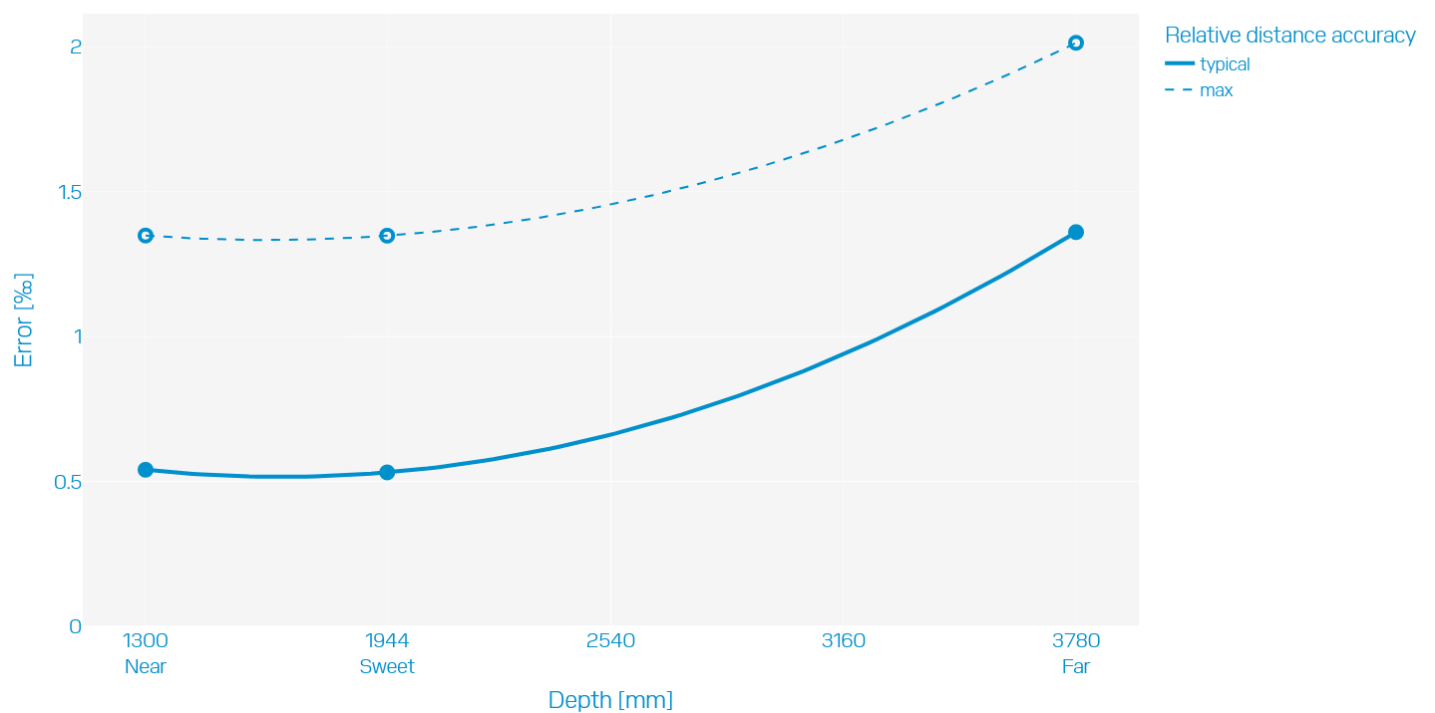
Relative distance accuracy - Camera mode MotionCam-3D L+
