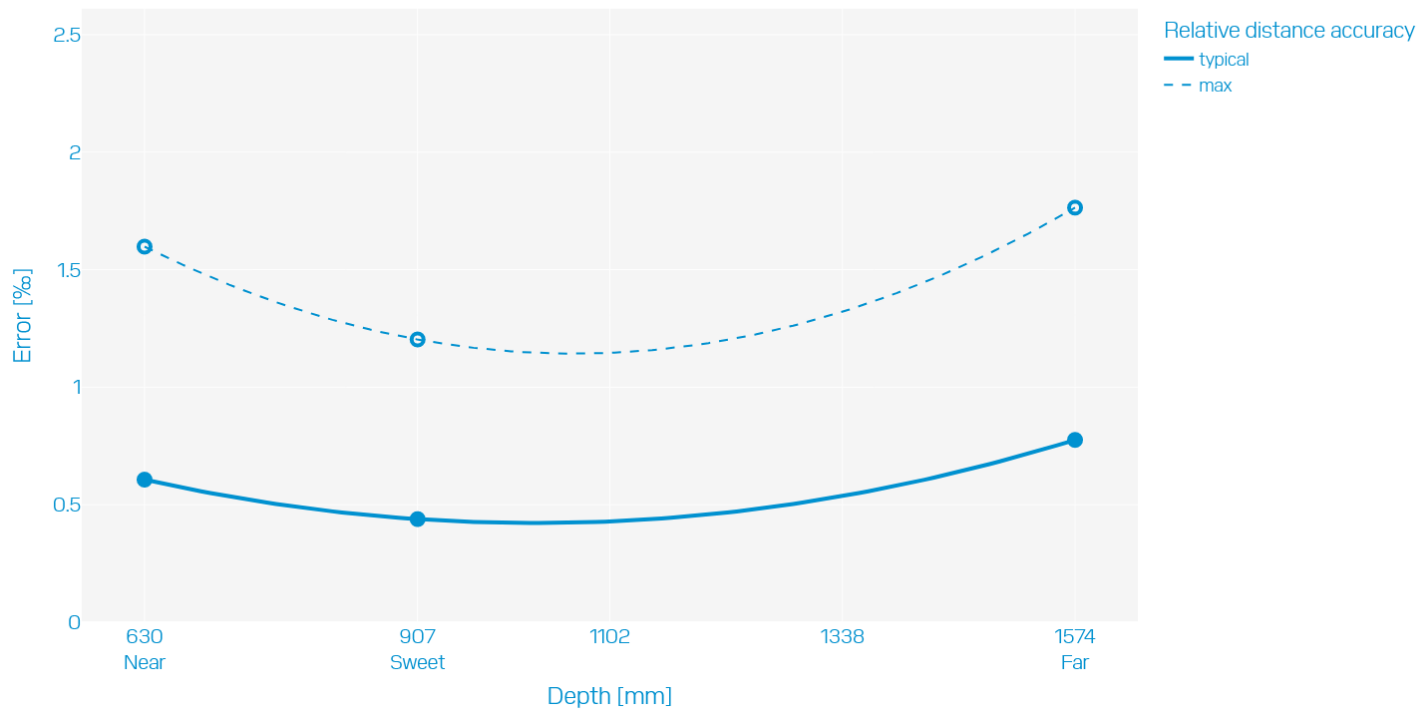
Relative distance accuracy - Scanner mode MotionCam-3D S+
