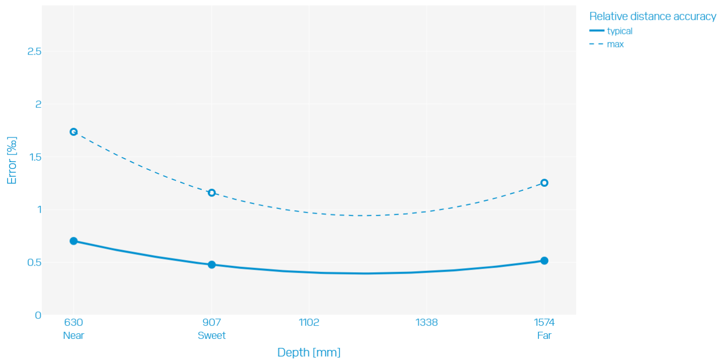
Relative distance accuracy - Scanner mode MotionCam-3D M+
