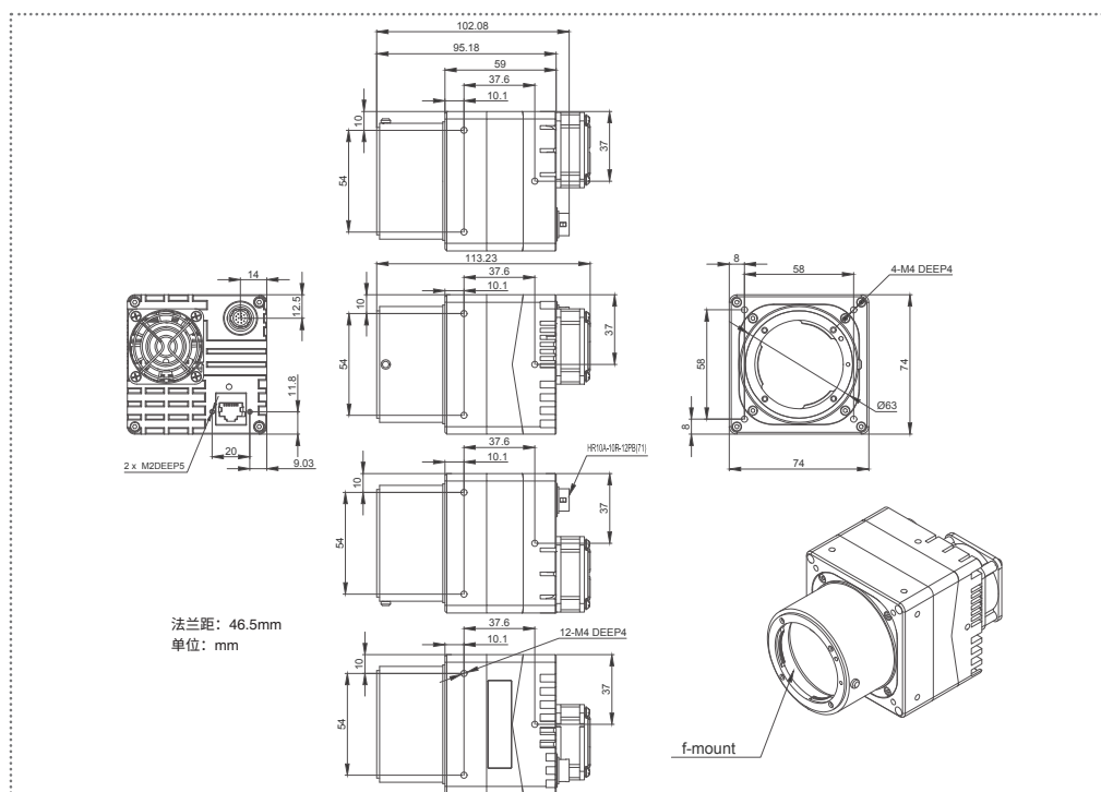
MARS-5000-24GTM/C-NF F, F □
